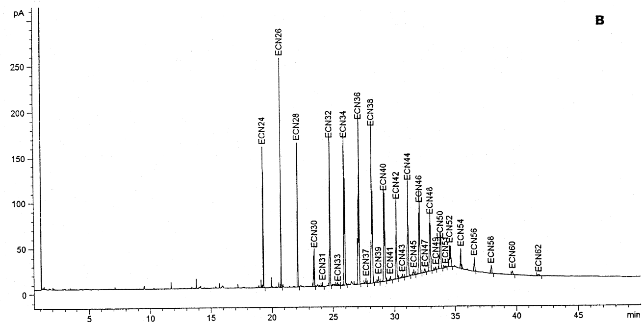
FIG. 3. Typical HTGC chromatogram of MCT and fish oil. (A) Physical mixture and (B) SL. See Figures 1 and 2 for abbreviations.
