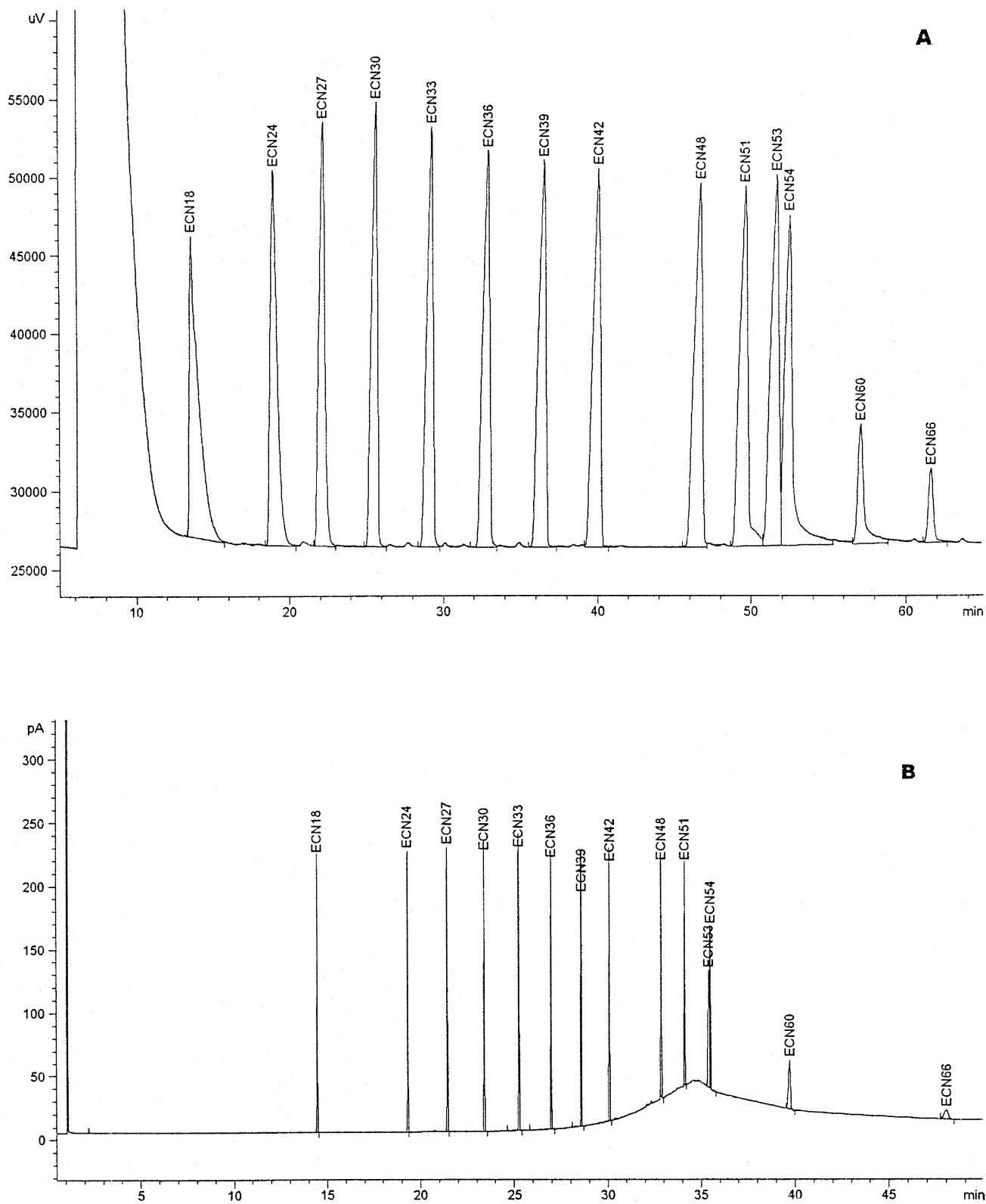
FIG. 1. Typical chromatogram of triacylglycerol standard mixture. (A) Supercritical fluid chromatography (SFC); (B) high-temperature gas chromatography (HTGC). ECN, equivalent carbon number.
