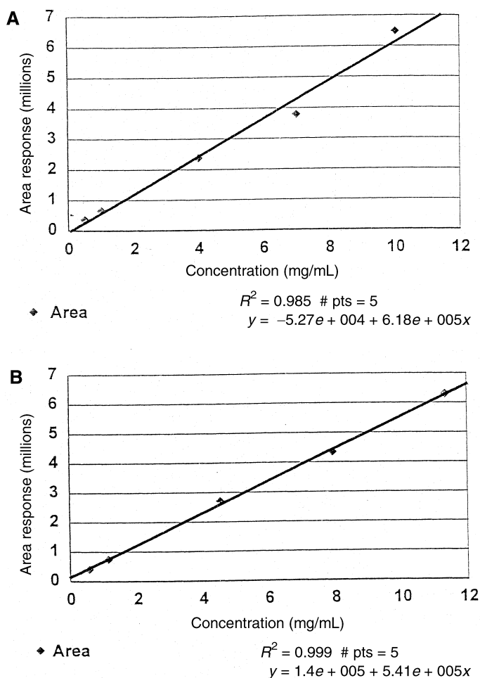
FIG. 4. Linear plot of detector response for SFC; (A) ECN 36 and (B) ECN 39. See Figures 1 and 2 for other abbreviation.
