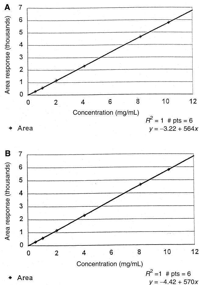
FIG. 5. Linear plot of detector response for HTGC; (A) ECN 36 and (B) ECN 39. See Figure 1 for abbreviations.
